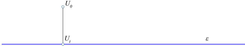
Figure 8: Calculate the distance |U_0 U_1| in barycentrics
