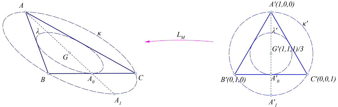
Figure 19: We see ABC and work with A'B'C'
